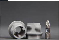
HIGH PRECISION, FINE DETAIL, FAST PRODUCTION METAL/CERAMIC: 316L, 17-4PH, COPPER, TOOL STEEL, TITANIUM, ALUMINA PLASTIC: PET-G, NYLON, PP, NYLON & PET CARBON OR GLASS FILLED
